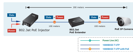
Figure 4: Connection architecture over 802.3at PoE Injector / POE-E201
