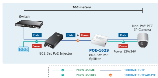
Figure 3: Connection architecture over 802.3at PoE Injector / POE-162S
