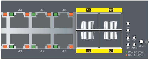
Figure 9-4: GS-4210-48T4S Reset Button
