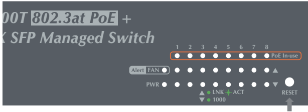
Figure 9-1: GS-4210-8P2S Reset Button
