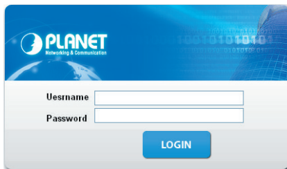
Figure 8-2: Login Screen
