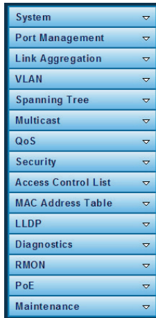
Figure 8-4: Switch Menu
