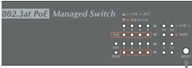
Figure 9-2: GS-4210-8P2T2S Reset Button
