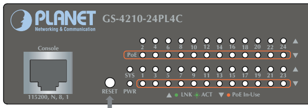
Figure 9-3: GS-4210-24P(L)4C Series Reset Button
