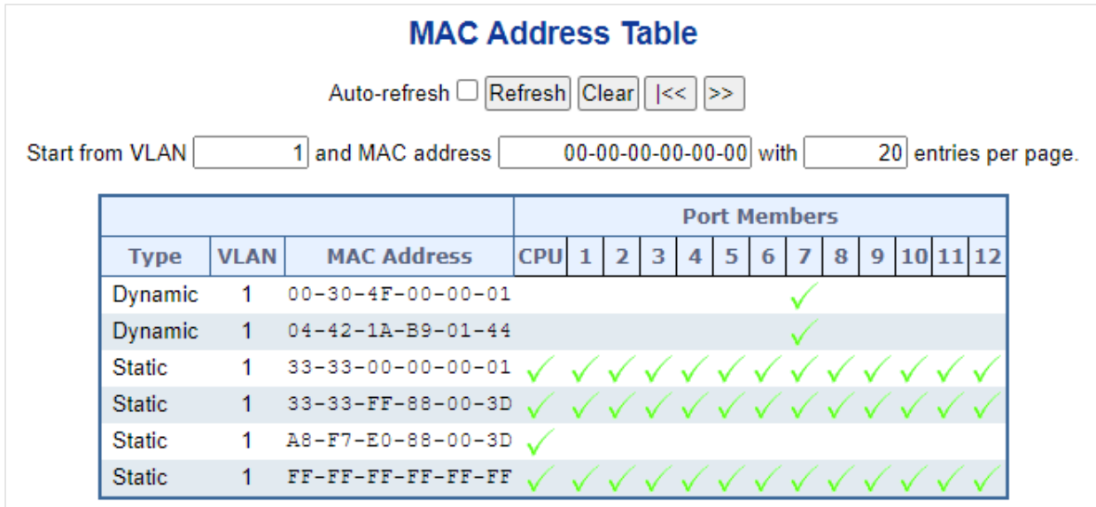
Figure 4-3-14-2: MAC Address Table Status Page Screenshot
