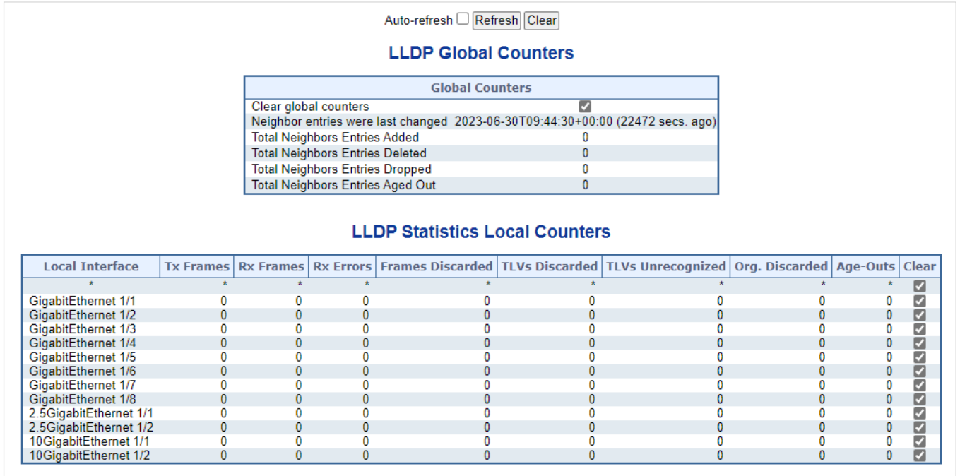
Figure 4-3-13-6: LLDP Statistics Page Screenshot
