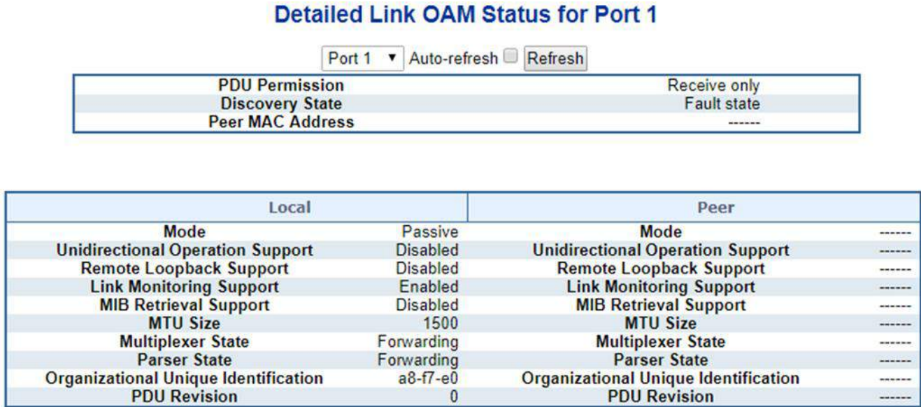
Figure 4-3-17-2: Port Status Page Screenshot
