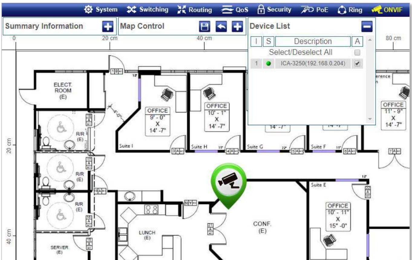
Figure 4-8-1-5: Floor Map Page Screenshot – add ONVIF IP camera from Device List
