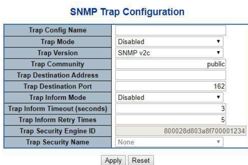
Figure 4-2-2-4: SNMP Trap Configuration Page Screenshot
