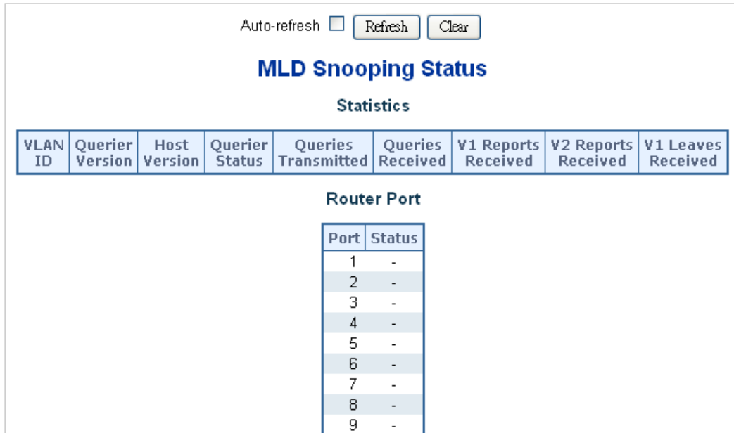
Figure 4-3-11-4: MLD Snooping Status Page Screenshot
