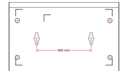
GSD-603F Switch Bottom Side
