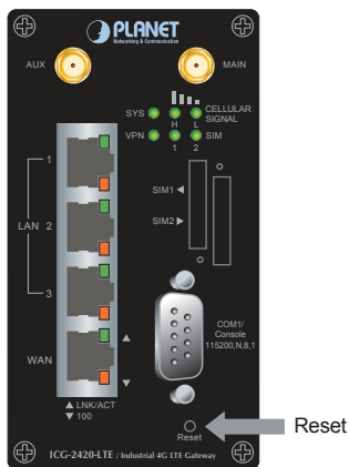
Figure 5-1: ICG-2420-LTE Reset Button
