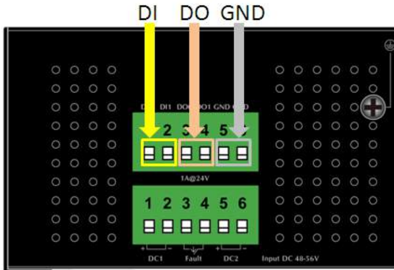
Figure 2-1-7a Wiring the Redundant Power Inputs
